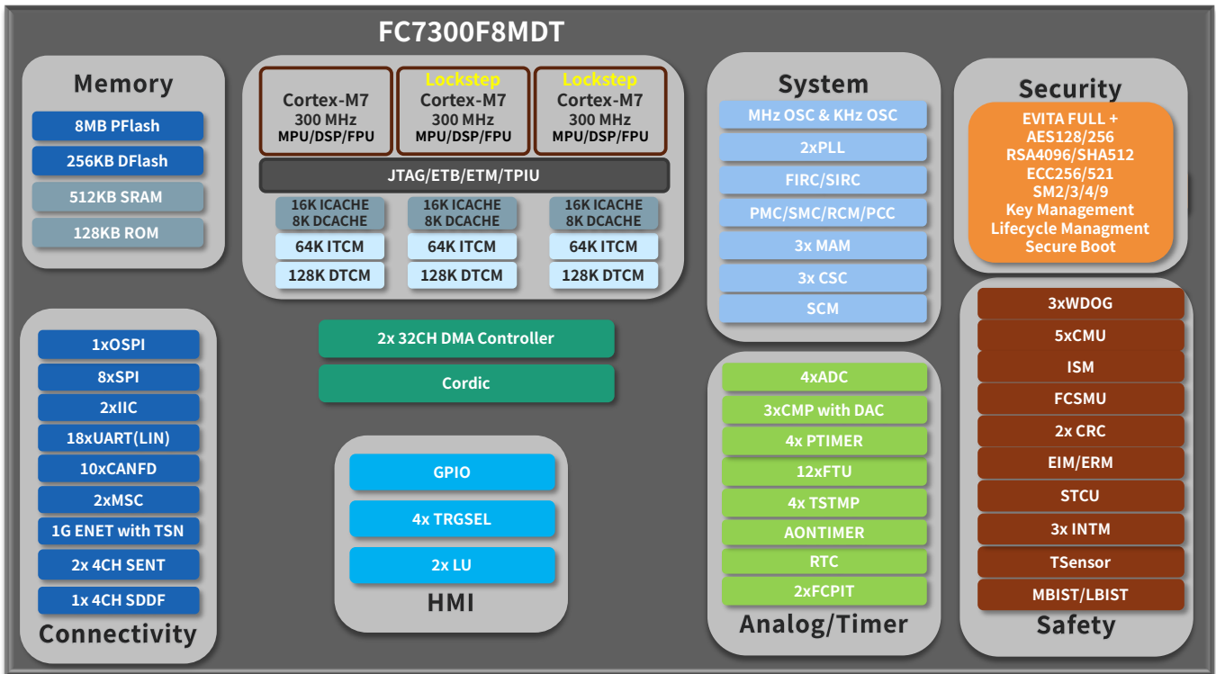
Figure 1. FC7300F8MDT block diagram
