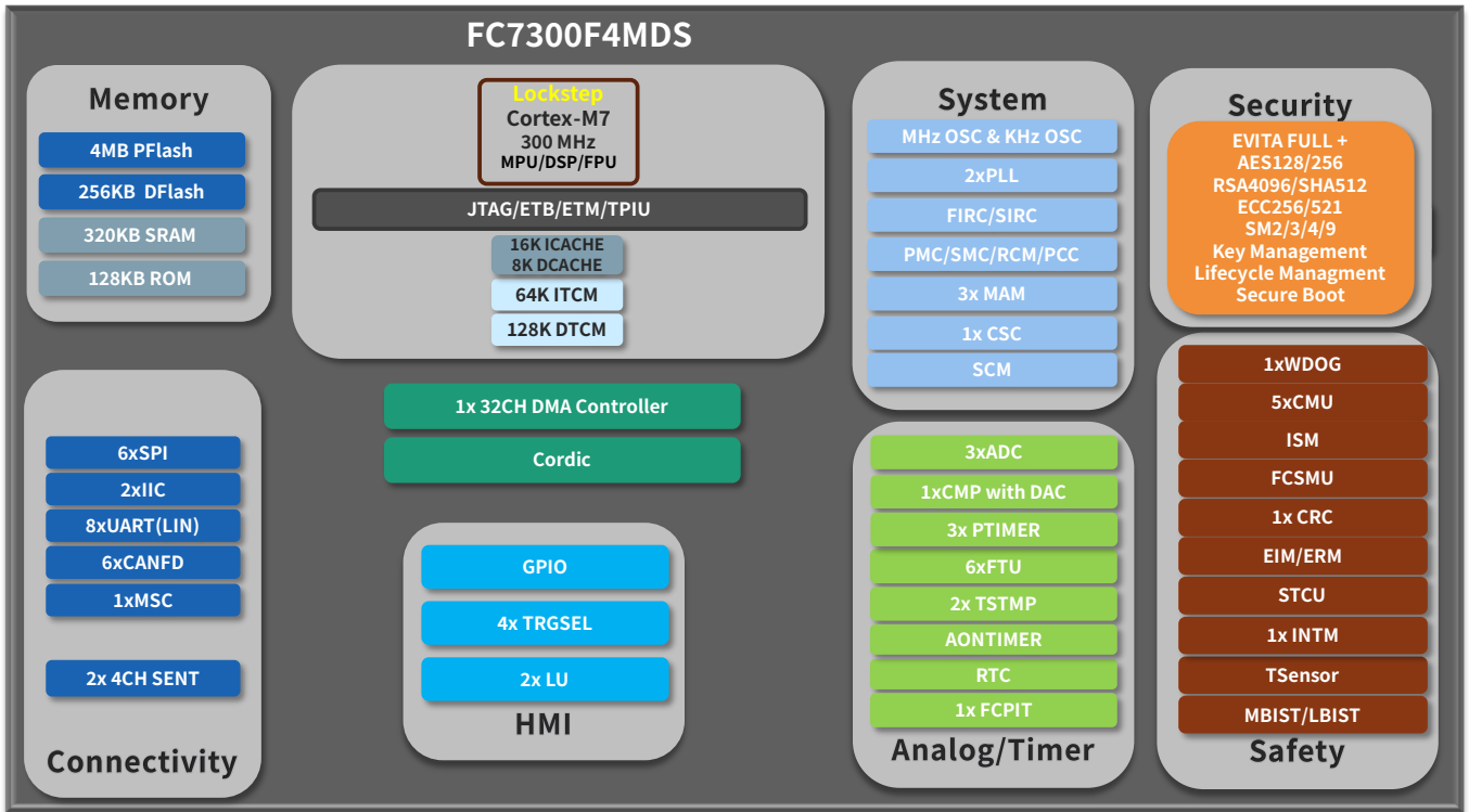
Figure 3. FC7300F4MDS block diagram
