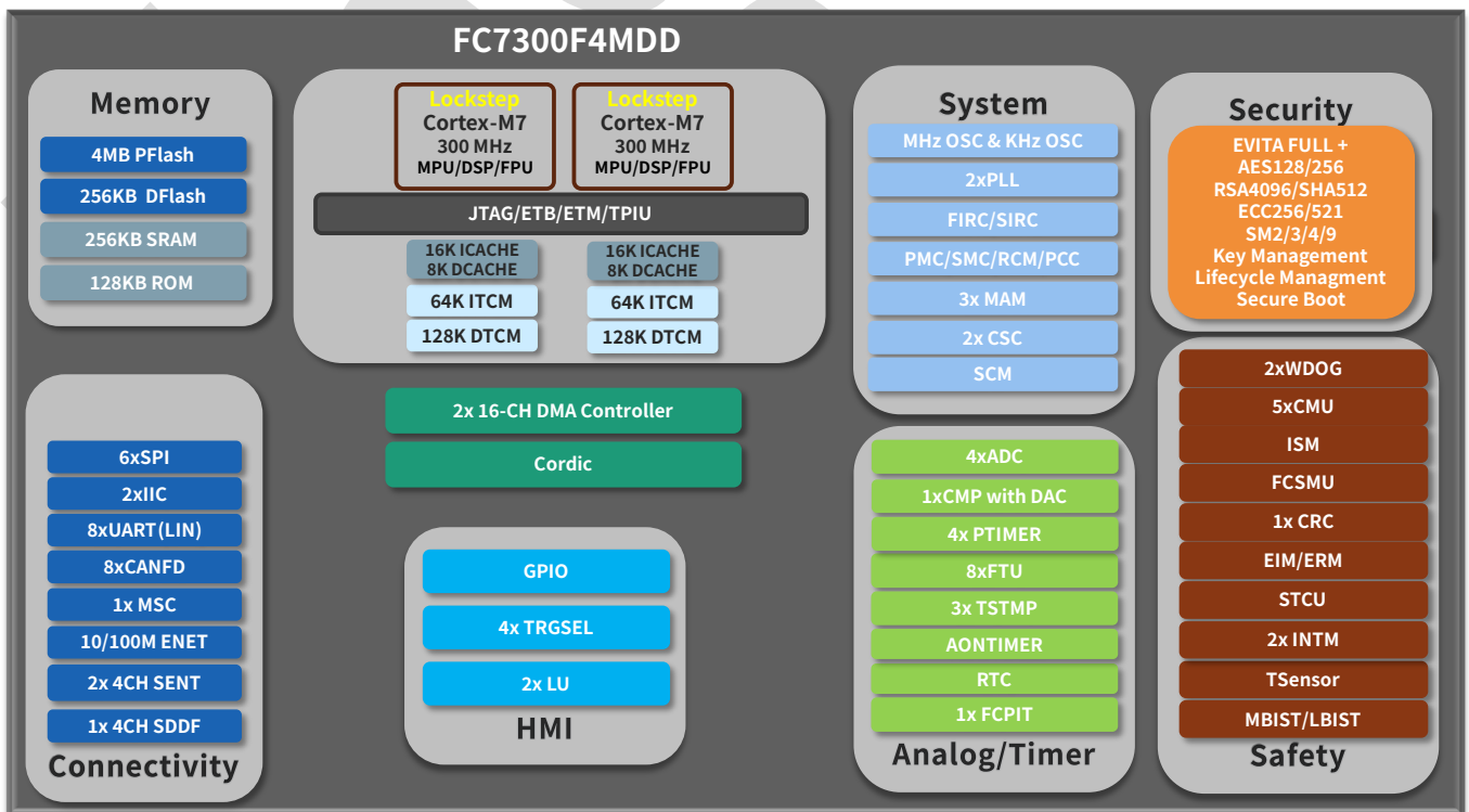
Figure 2. FC7300F4MDD block diagram
